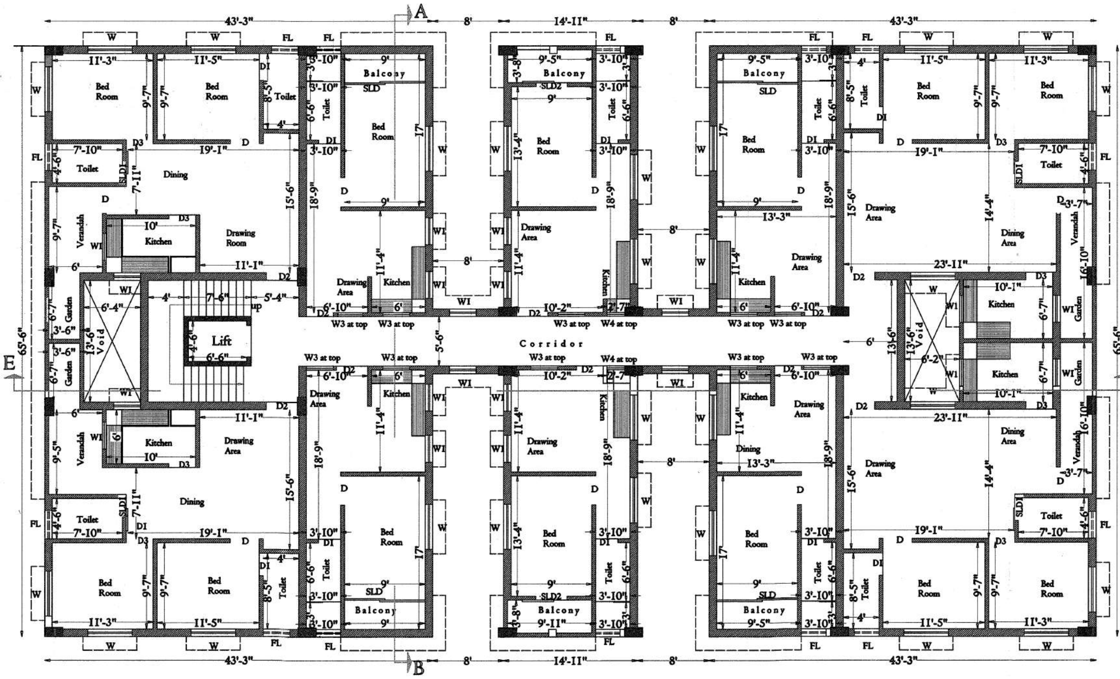
Typical Floor Plan 1st to 4th
